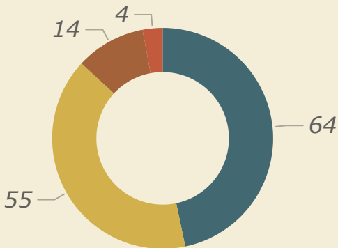
Formats Read
